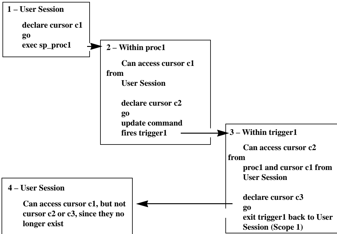
Figure 1-1: How cursors operate within scopes
